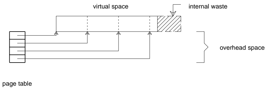
Figure 3.12 Wasted space and page size
