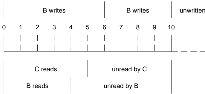
Figure 9.3 Reads and writes on a broadcast pipe
