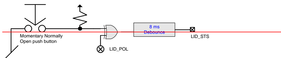
Figure 4-19 Example Generic Address Space Lid Switch Logic
