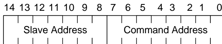
Figure 15-2 SMBus Linear Address Decode
