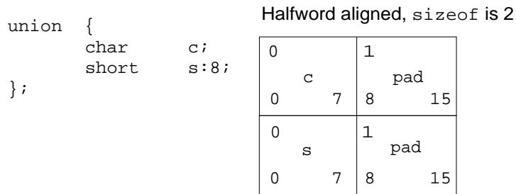
Figure 3-22 union Allocation—Big-Endian
