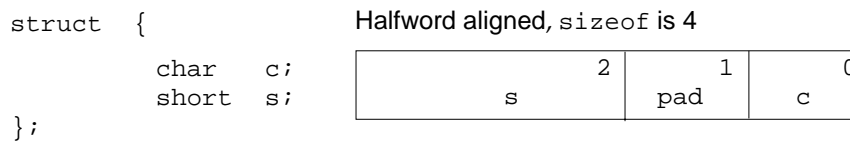
Figure 3-8 Internal Padding—Little-Endian
