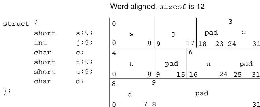
Figure 3-18 Boundary Alignment—Big-Endian
