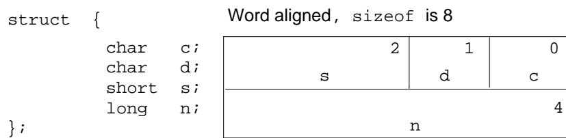
Figure 3-6 No Padding—Little-Endian
