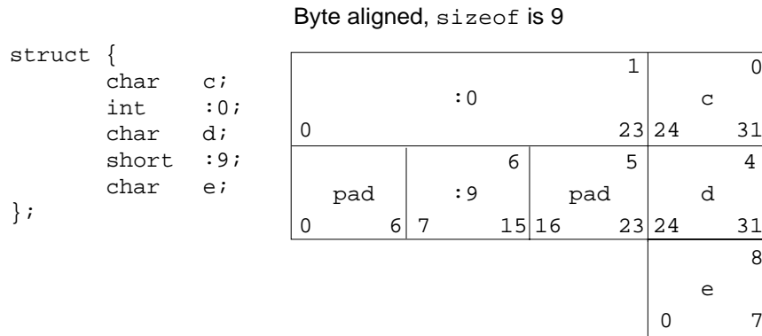
Figure 3-23 Unnamed Bit-Fields—Little-Endian
