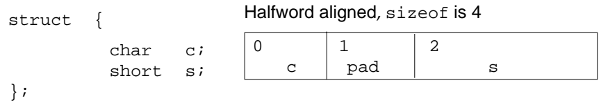
Figure 3-9 Internal Padding—Big-Endian
