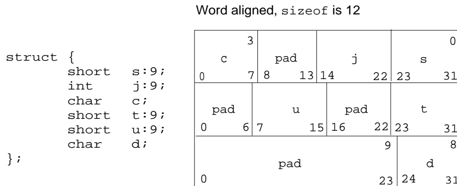
Figure 3-17 Boundary Alignment—Little-Endian
