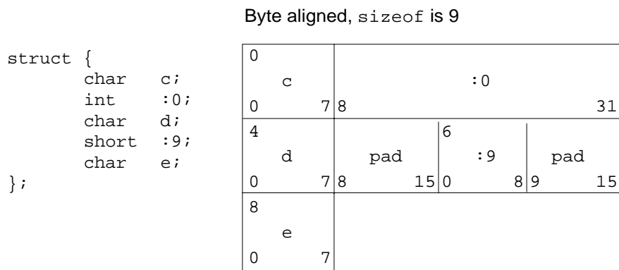
Figure 3-24 Unnamed Bit-Fields—Big-Endian
