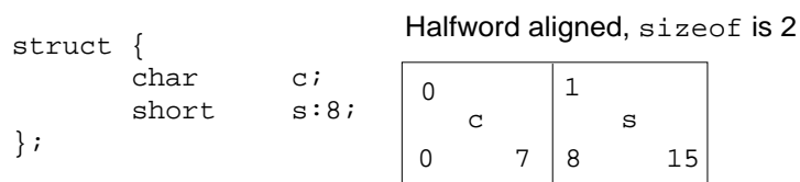
Figure 3-20 Storage Unit Sharing—Big-Endian
