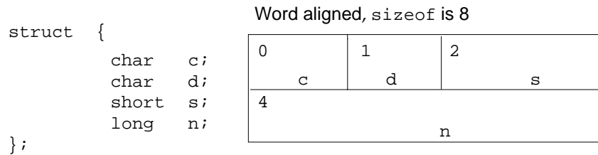
Figure 3-7 No Padding—Big-Endian
