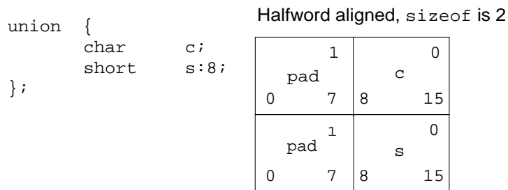
Figure 3-21 union Allocation—Little-Endian
