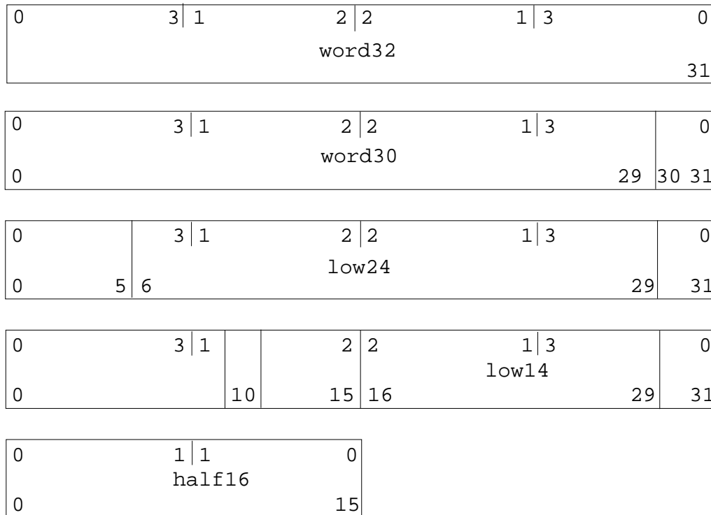
Figure 4-1 Relocation Fields
