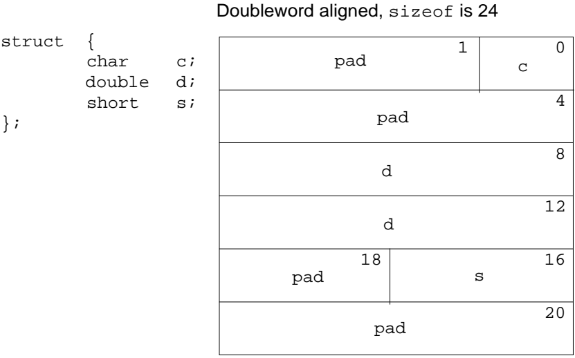
Figure 3-10 Internal and Tail Padding—Little-Endian
